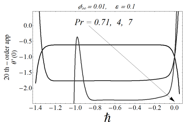
Figure 2. \hbar - Curves for the temperature function \theta against different values of the Prandtl number Pr plotted for the 20 th order approximation of the HAM solutions when k_1 = 0.5, Gr = 1, Mn = 0.5, Nr = 0.2, Nr^* = 0.2, Nt = 0.5, Nb = 0.25, Sc = 1 .
