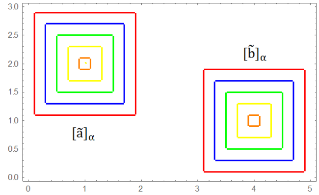
Figure 2. [\tilde{a}]_{\alpha} and [\tilde{b}]_{\alpha} .
